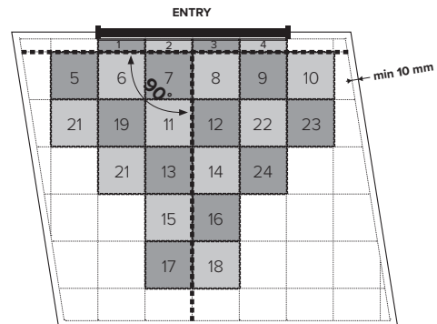
Fig. 2 Installing Fortelock INVISIBLE, BUSINESS
