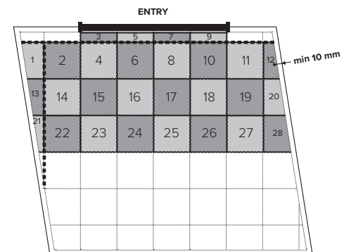
Fig. 3 Direction of installing INVISIBLE, BUSINESS
